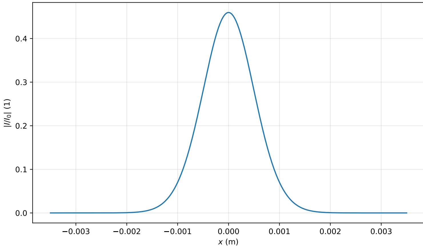
Intensity profile I(x, y = 0, z = 2.548m)/I_0 , P_{in}=0.2P_{cr} , artificial time
